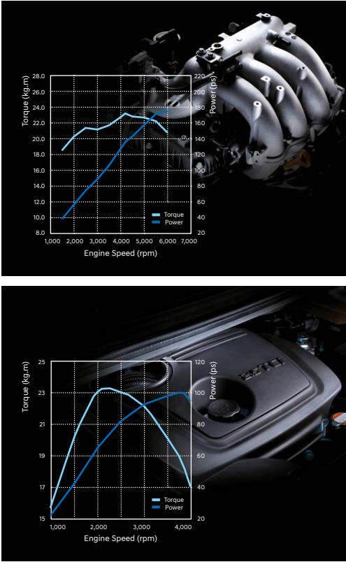
2.4 MPi gasoline engine 2.5 TCi diesel engine
